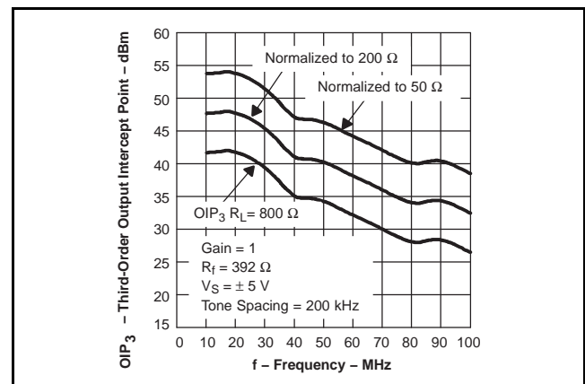
Figure 109. Equivalent 3rd-Order Intercept Point for the THS4500
